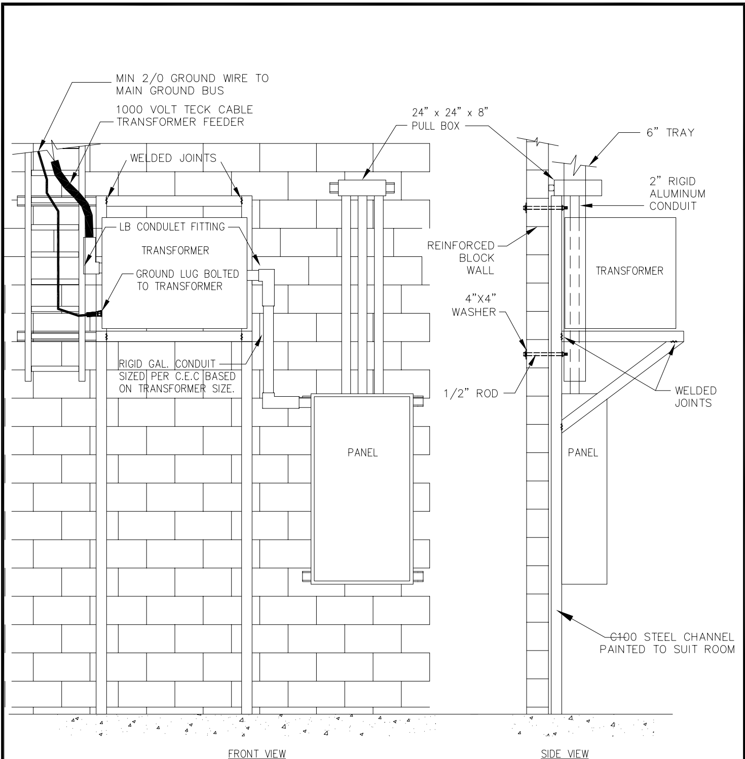
FRONT VIEW
